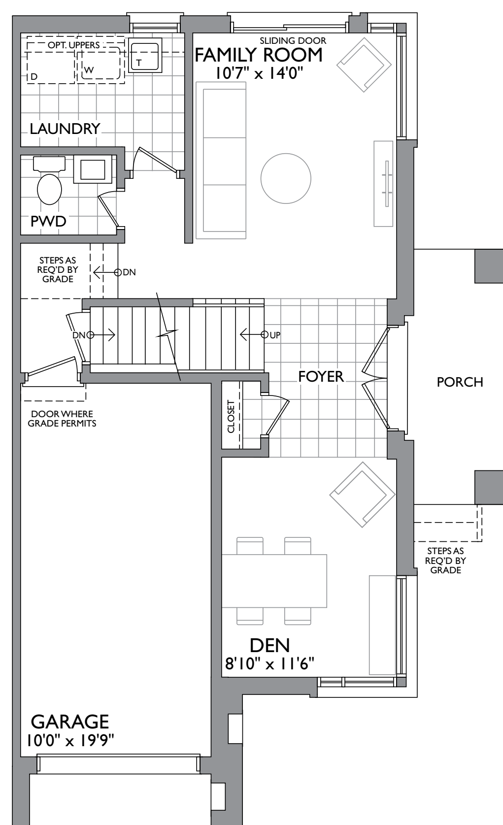
FIRST FLOOR
