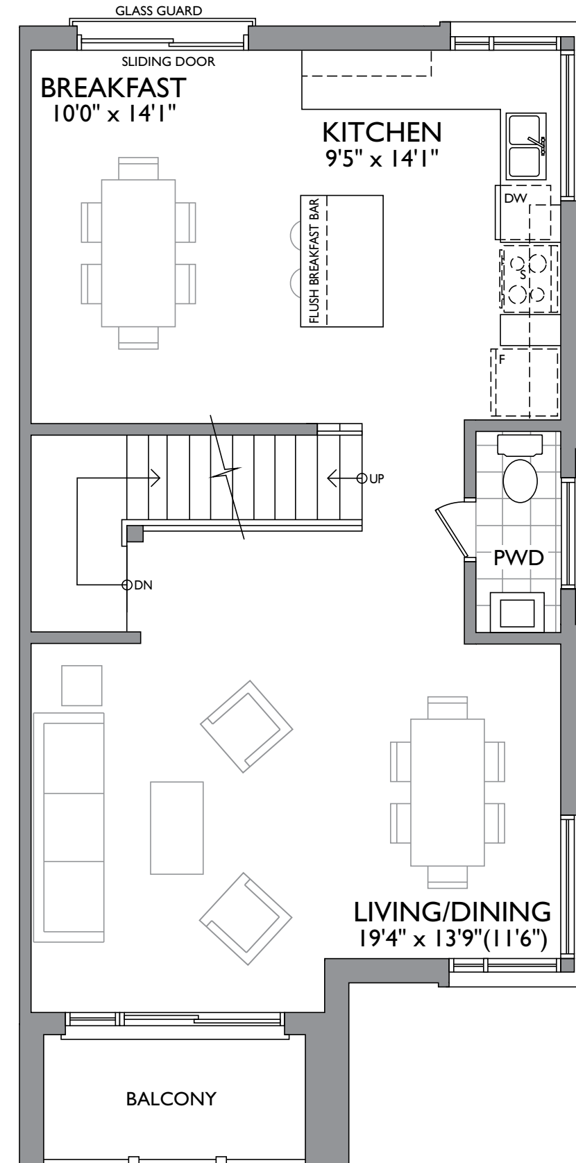
SECOND FLOOR
